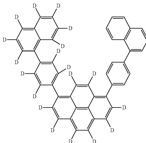
Formula IIa
